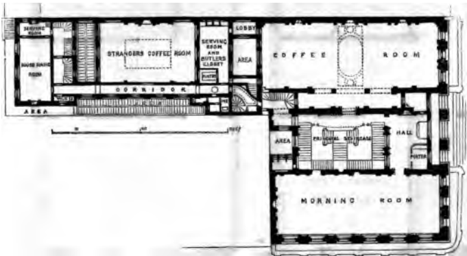
PLAN OF ARMY AND NAVY CLUB-HOUSE.
